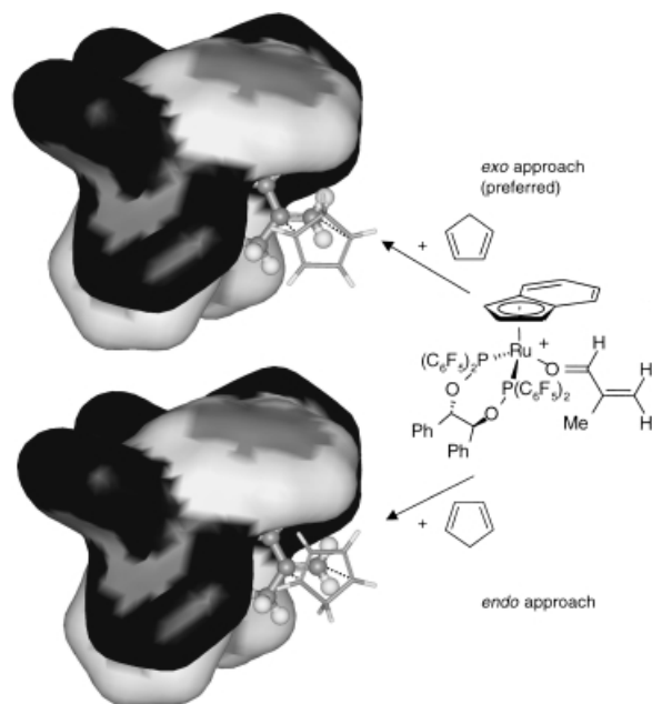
Figure 3. Model of the transition state for the Diels–Alder reaction of methacrolein and cyclopentadiene catalyzed by (S,S)-5d. Top: cyclopentadiene exo approach to the methacrolein C α -Re face. Bottom: cyclopentadiene endo approach to the methacrolein C α -Re face.
